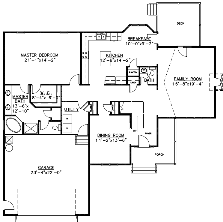
FIRST FLOOR PLAN 1690 SQ. FT. All room dimensions shown are approximate.
