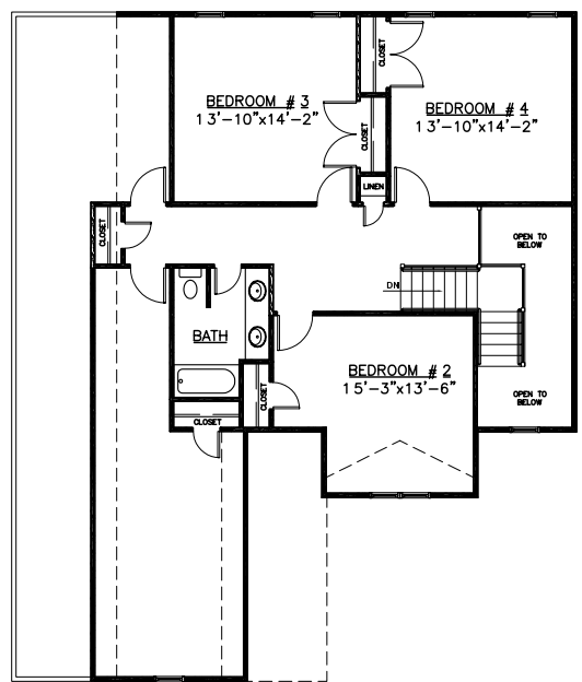
SECOND FLOOR PLAN 1252 SQ. FT. All room dimensions shown are approximate.
