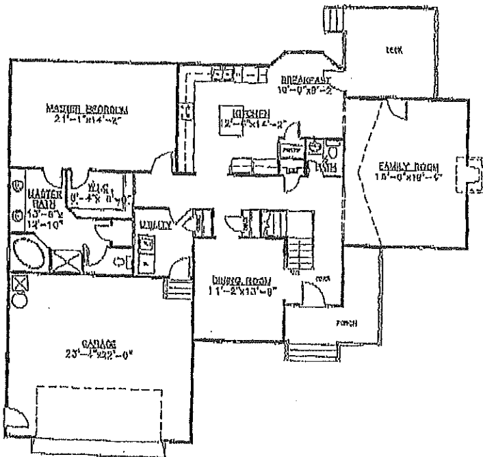
FIRST FLOOR PLAN All room dimensions shown are approximate.
